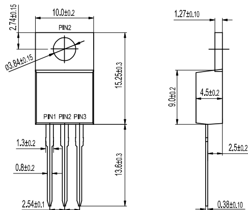
TO-220AB FR12XXCT
